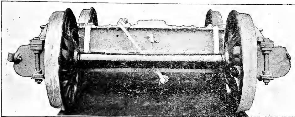
Fig. 4577. End View. FREIGHT-CAR TRUCK. HARVEY STEEL CAR & REPAIR WORKS, HARVEY, ILL.
